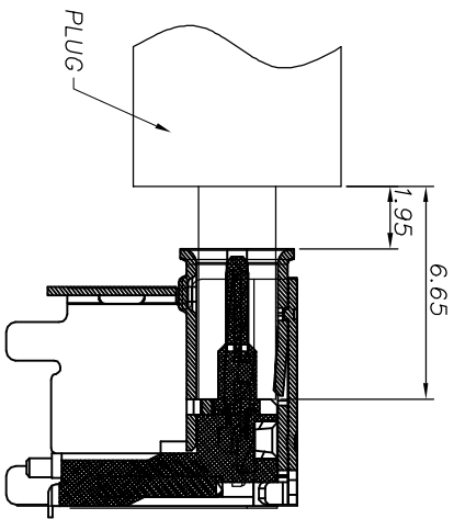
AFTER MATING
